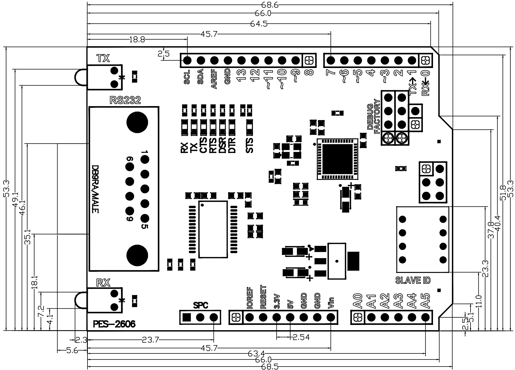
PES-2606 Dimension (mm)
